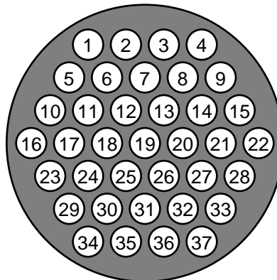
Figure 1: The CPC connector for the relay card.
